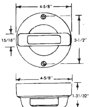
Surface Mounting Unit for Exposed Wiring
